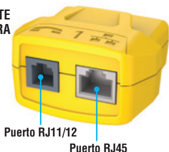
Puerto RJ45
